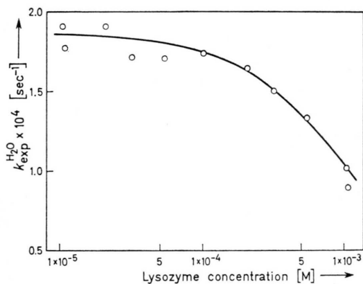
Fig. 5. Protein dependence of k_{exp} in H_2O (acridine orange 1 \times 10^{-4} M, phosphate buffer pH 5.9 ( I=0.07 ), PIL 492 nm).
