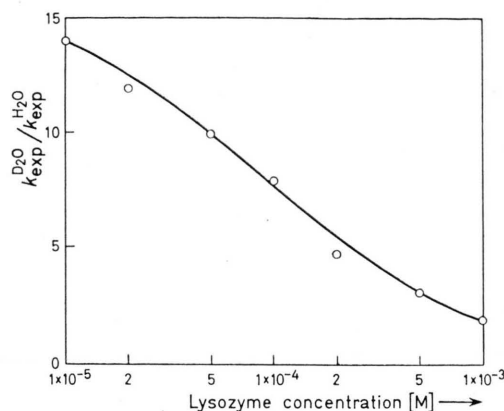
Fig. 7. k_{\text{exp}}^{\text{D}_2\text{O}}/k_{\text{exp}}^{\text{H}_2\text{O}} in dependence of the lysozyme concentration.
