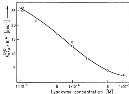
Fig. 6. Protein dependence of k_{exp} in D_2O (acridine orange 1 \times 10^{-4} M, phosphate buffer pD 5.9 ( I=0.07 ), PIL 492 nm).
