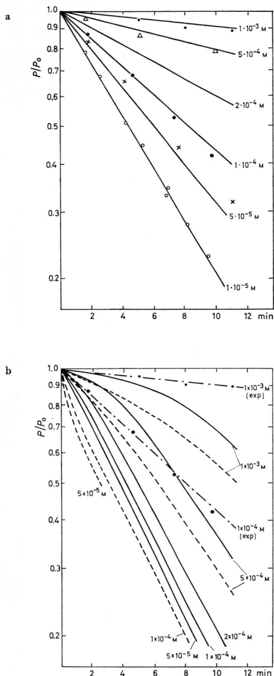
Fig. 9. Decrease of the enzymatic activity with time of exposure (492 nm). Dependence of the kinetics upon the lysozyme concentration. Solvent: phosphate buffer pH 5.9 ( D_2O , air saturated) acridine orange 1 \times 10^{-4} M . Lysozyme = 1 \times 10^{-3} M (●), 5 \times 10^{-4} M (△), 1 \times 10^{-4} M (●), 5 \times 10^{-5} M (×), 1 \times 10^{-5} M (○). Analog computation: (a) k_6 = 3.9 \times 10^7 M^{-1} sec^{-1} , k_7^0 = 4.2 \times 10^8 M^{-1} sec^{-1} , k_7^* = 0 (solid lines), (b) k_6 = 3.9 \times 10^7 M^{-1} sec^{-1} , k_7^0 = 0 , k_7^* = 4.2 \times 10^8 M^{-1} sec^{-1} activity of P' = 100\% (solid lines), 80% (dashed lines).
